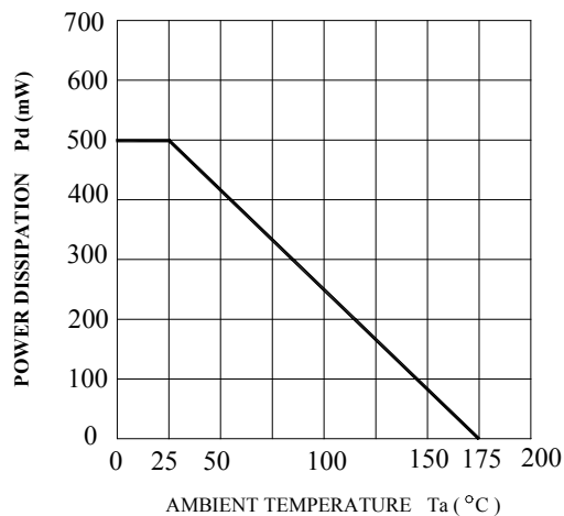
Fig. 2 Derating curve
