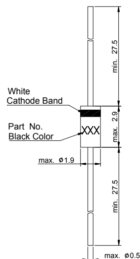
Glass case JEDEC DO-34 Dimensions in mm
